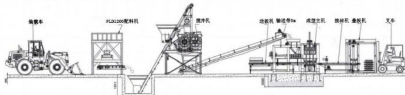
地基图 GROUNDWORK DRAWING
